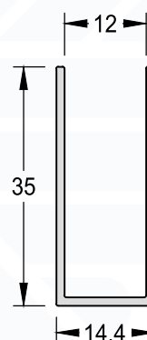
Arremate "U"
