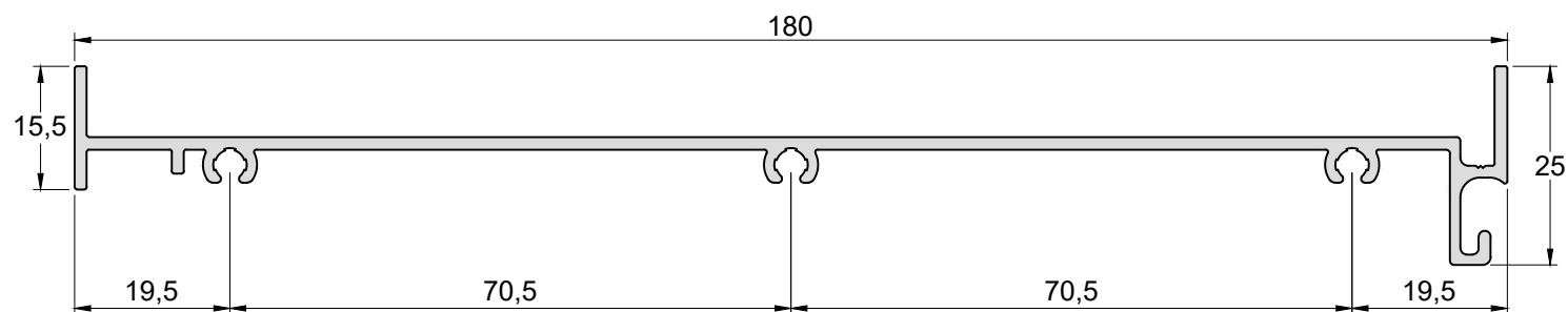
Marco Superior Horizontal TL-044 1,089 kg/m
