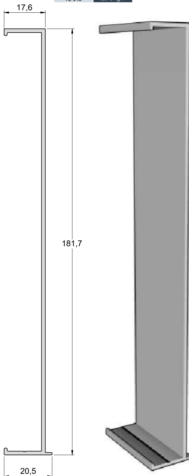
Marco Lateral Vertical TL-043 0,943 kg/m
